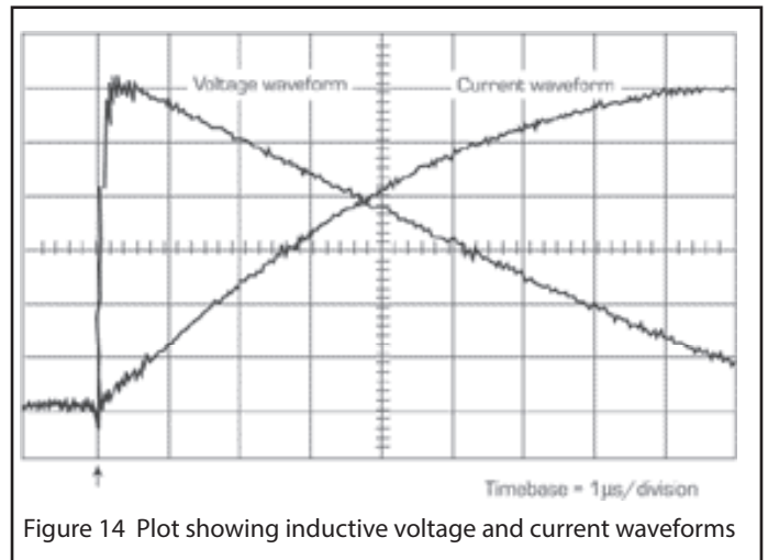
Figure 14 Plot showing inductive voltage and current waveforms
