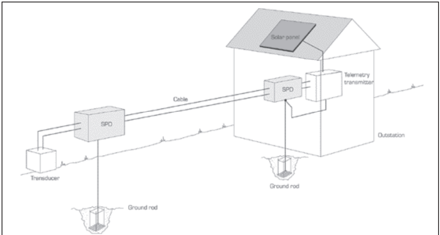
Figure 34 Outstation installation – with ground rod
