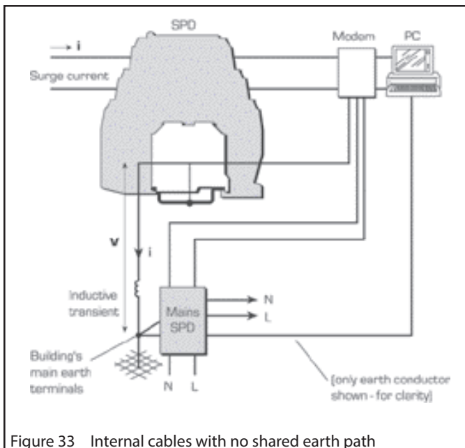
Figure 33 Internal cables with no shared earth path
