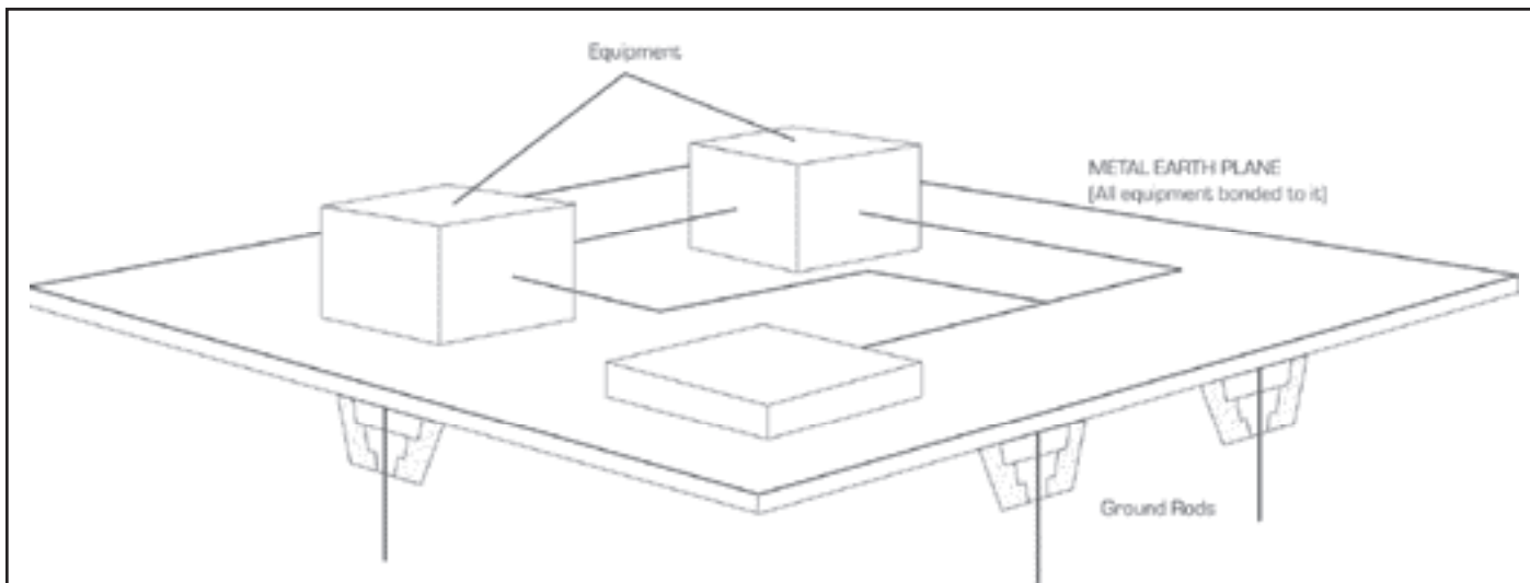
Figure 5 A less than 'ideal' system
