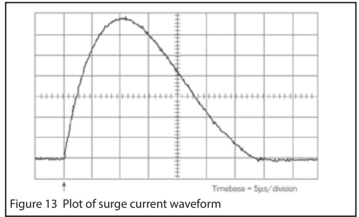
Figure 13 Plot of surge current waveform
